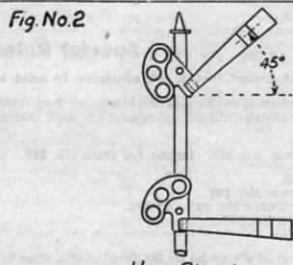
Home Signal Color Upper Arm YELLOW light at night. Lower Arm RED light at night. Indication Proceed on main line with caution, prepared to stop at the Block Station. Name CAUTION Signal.
