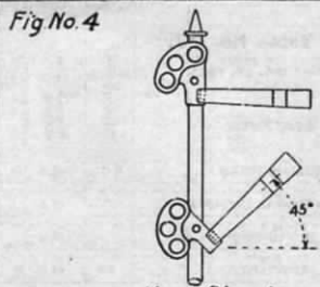
Home Signal Color Upper Arm RED light at night. Lower Arm YELLOW light at night. Indication Take Passing Track. Name CAUTION signal.
