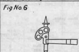
Distant Signal Color RED light at night. Indication STOP then proceed with caution to home signal. Name STOP Signal.
